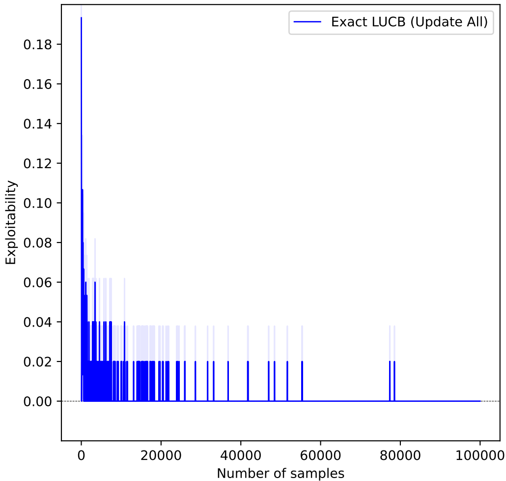
Kuhn Poker, PAC, \epsilon = 0.01 , \delta = 0.01 , Player o
